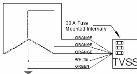
Buss Connection
