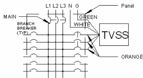
Panel Connection
