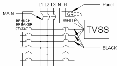
Panel Connection
